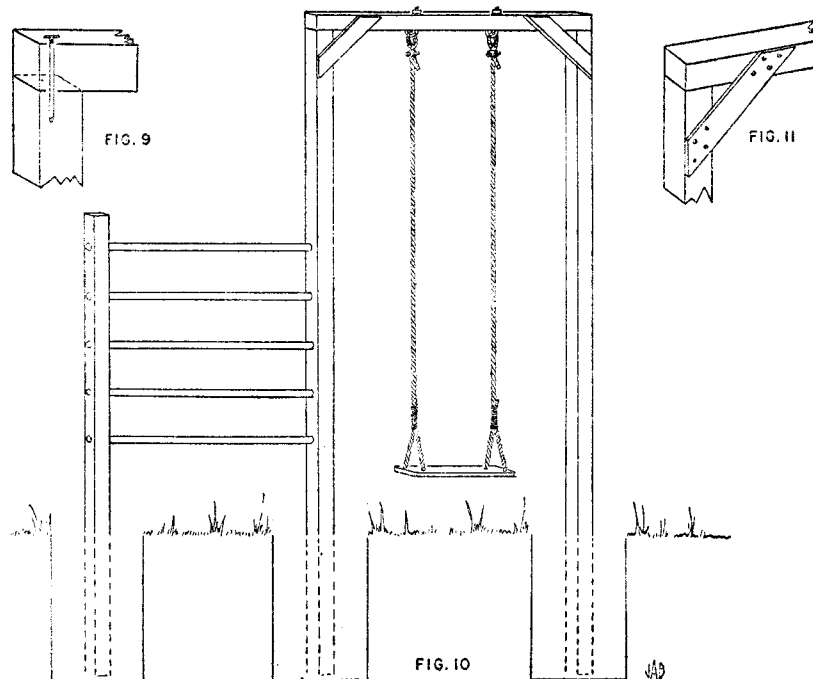
CONSTRUCTION OF FRAME
